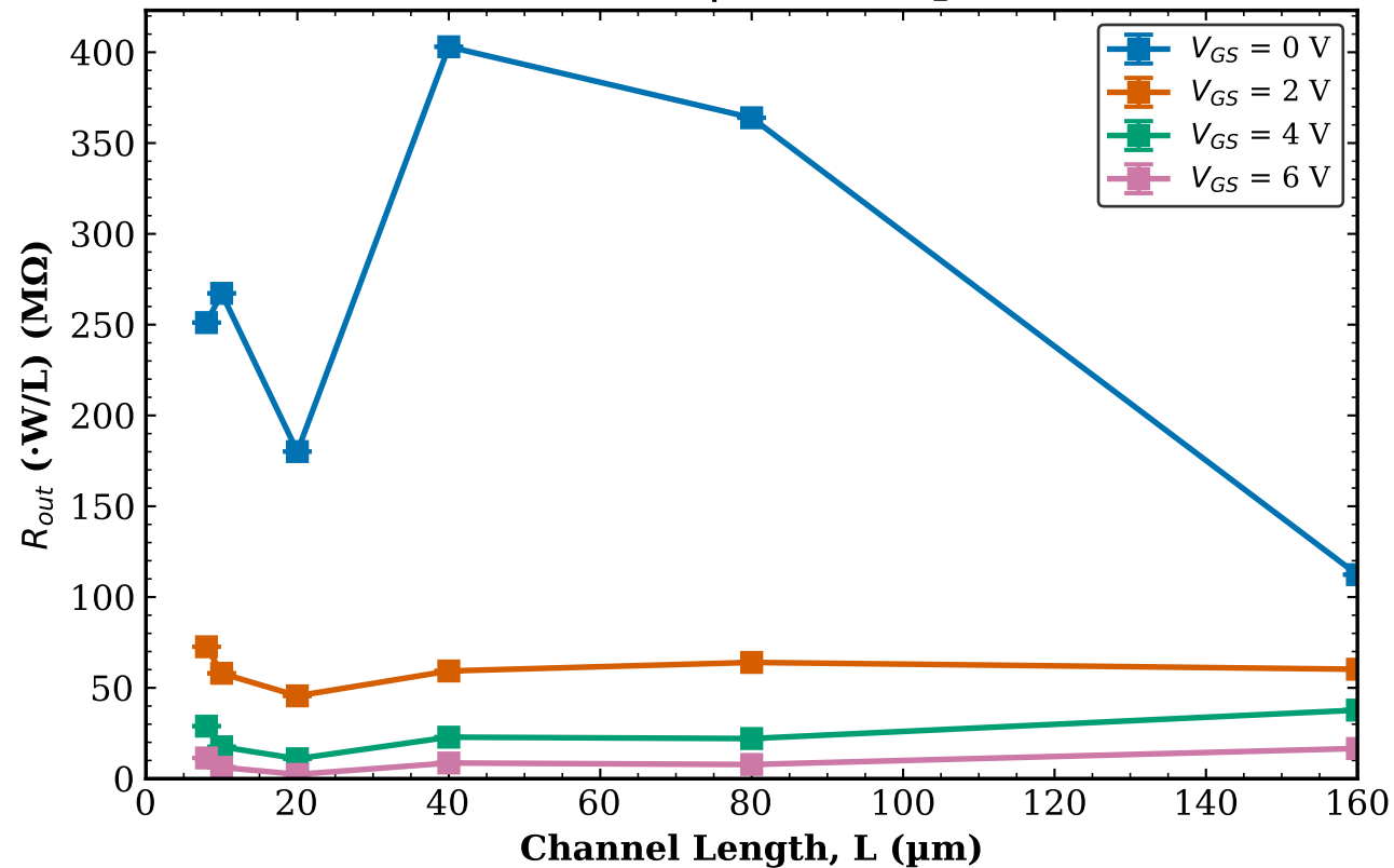
TFT1 Transistor 2 R_{out} vs L | W = 10\text{ }\mu\text{m}
